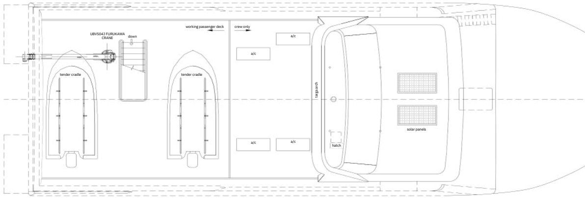
SUN DECK
