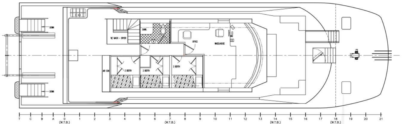
WHEELHOUSE DECK
